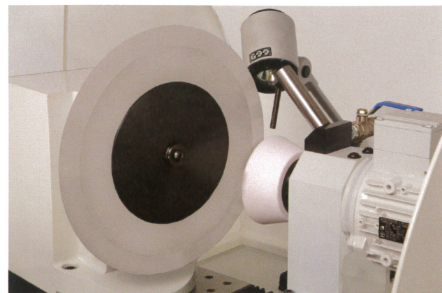
Grinding example of bowl-shaped grinding wheel カップ砥石研磨例
