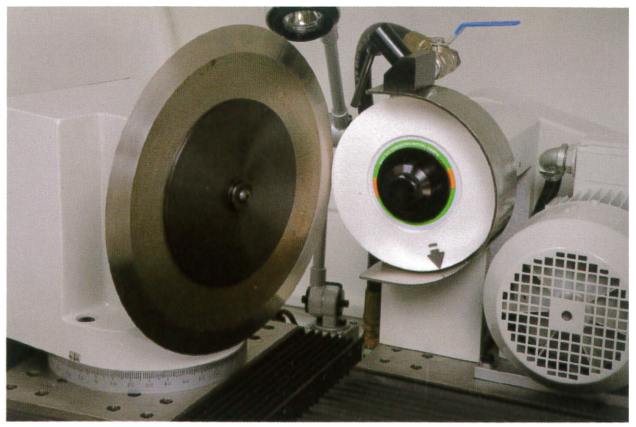
Grinding example of plane grinding wheel 平型砥石研磨例
